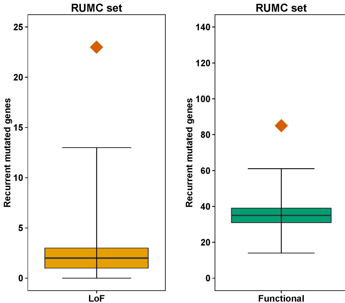
Supplementary Figure 5. Simulations of recurrently mutated genes of the RUMC cohort.
